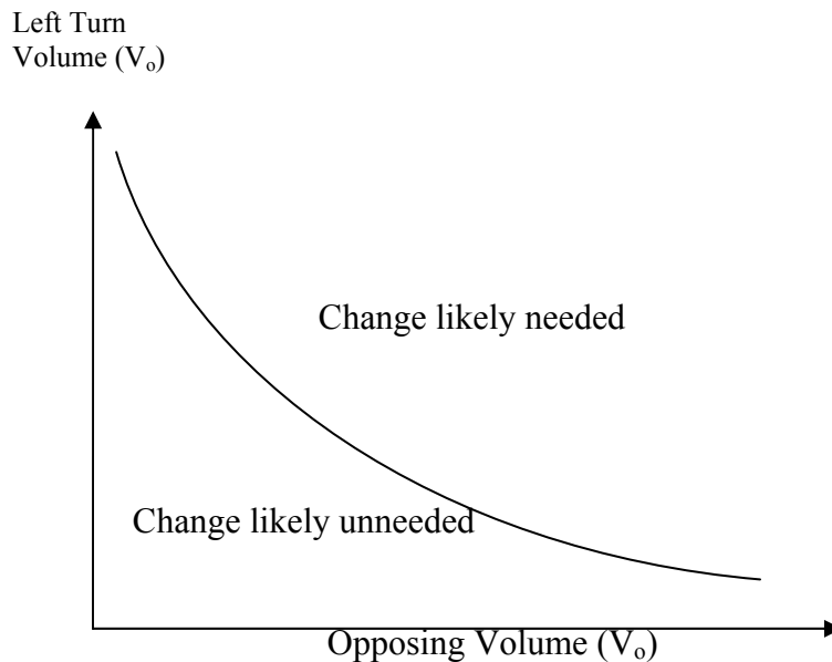
Figure 7-1: Concept of the Assessment Tool
