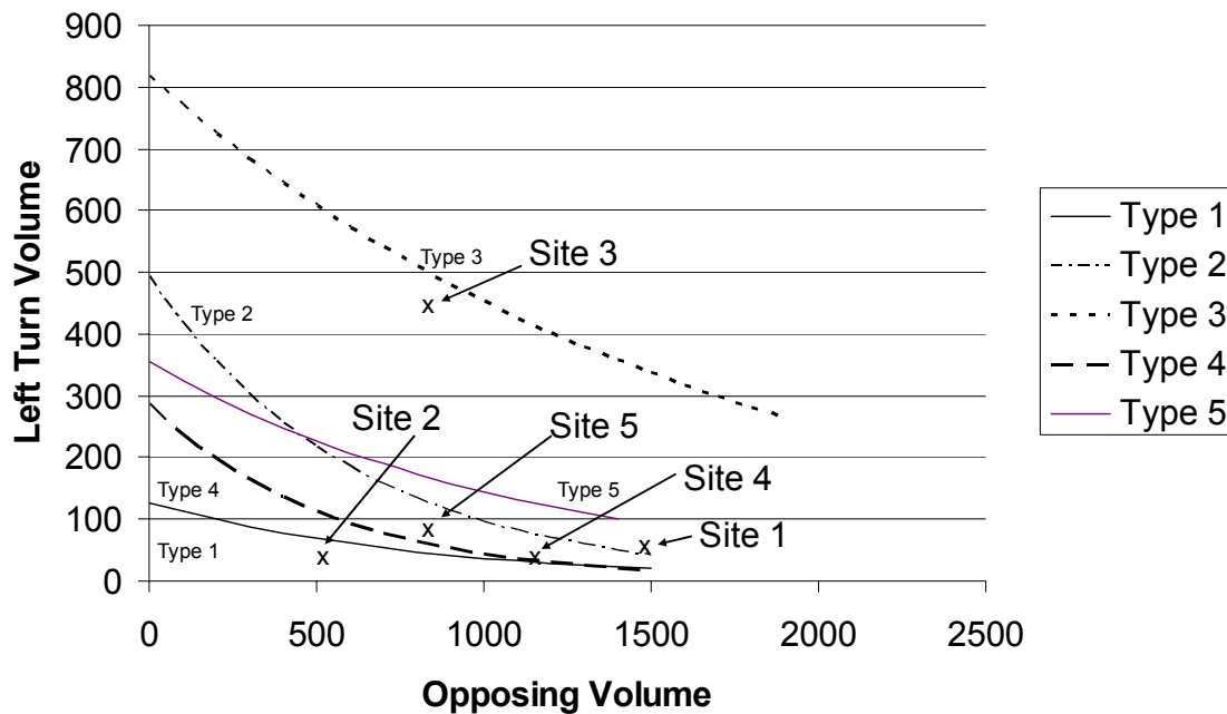
Figure 7-5. Application of Decision Tool to Five Sites
